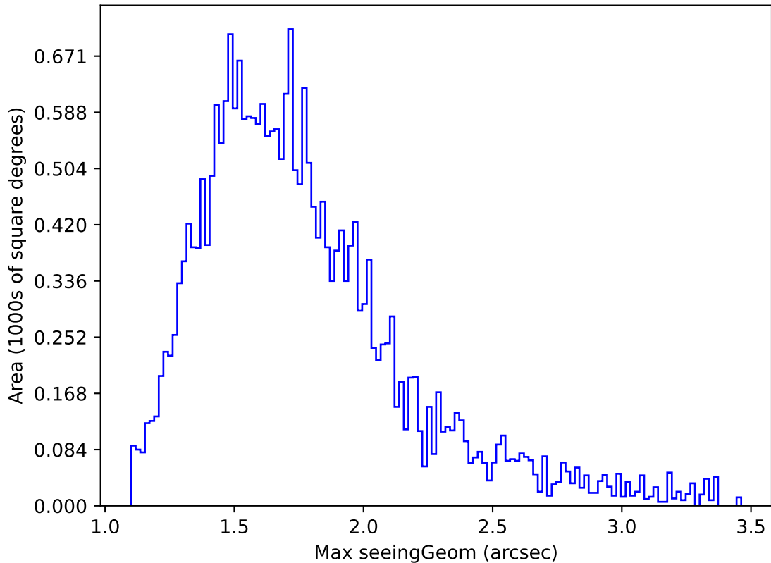
too_elab_r64_d2_gz_v3.4_10yrs Yr 1 all bands: Max seeingGeom
