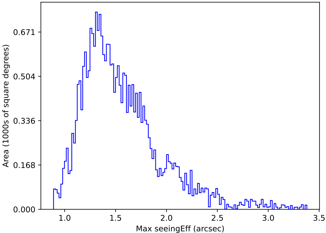
too_elab_r64_d2_gz_v3.4_10yrs Yr 1 z band: Max seeingEff
