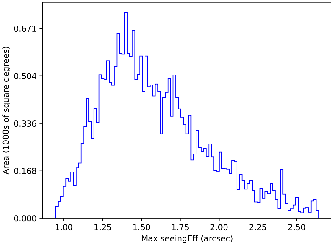
too_elab_r64_d2_gz_v3.4_10yrs Yr 1 r band: Max seeingEff
