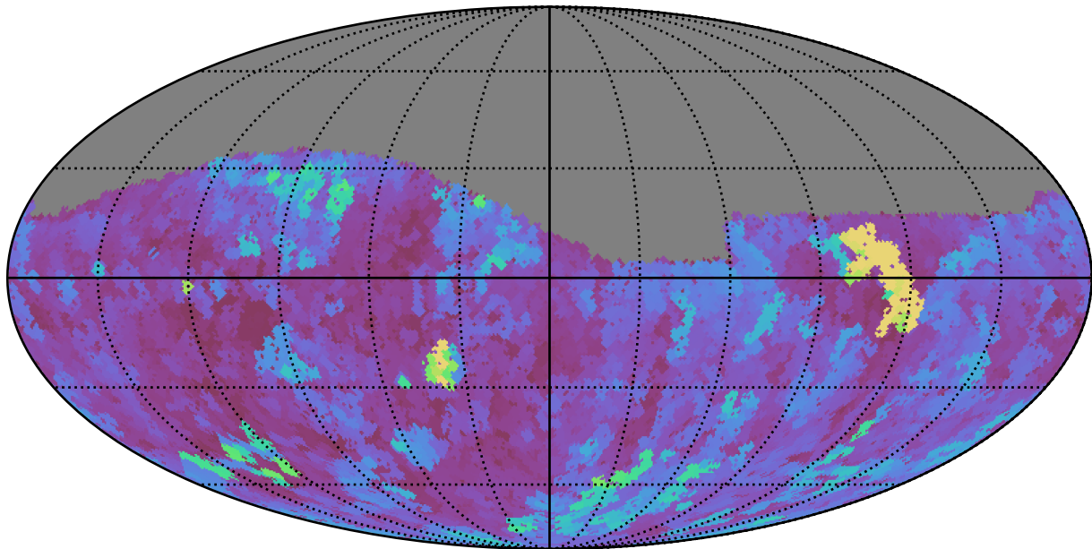
too_elab_r64_d2_gz_v3.4_10yrs Yr 1 g band: Max seeingEff
