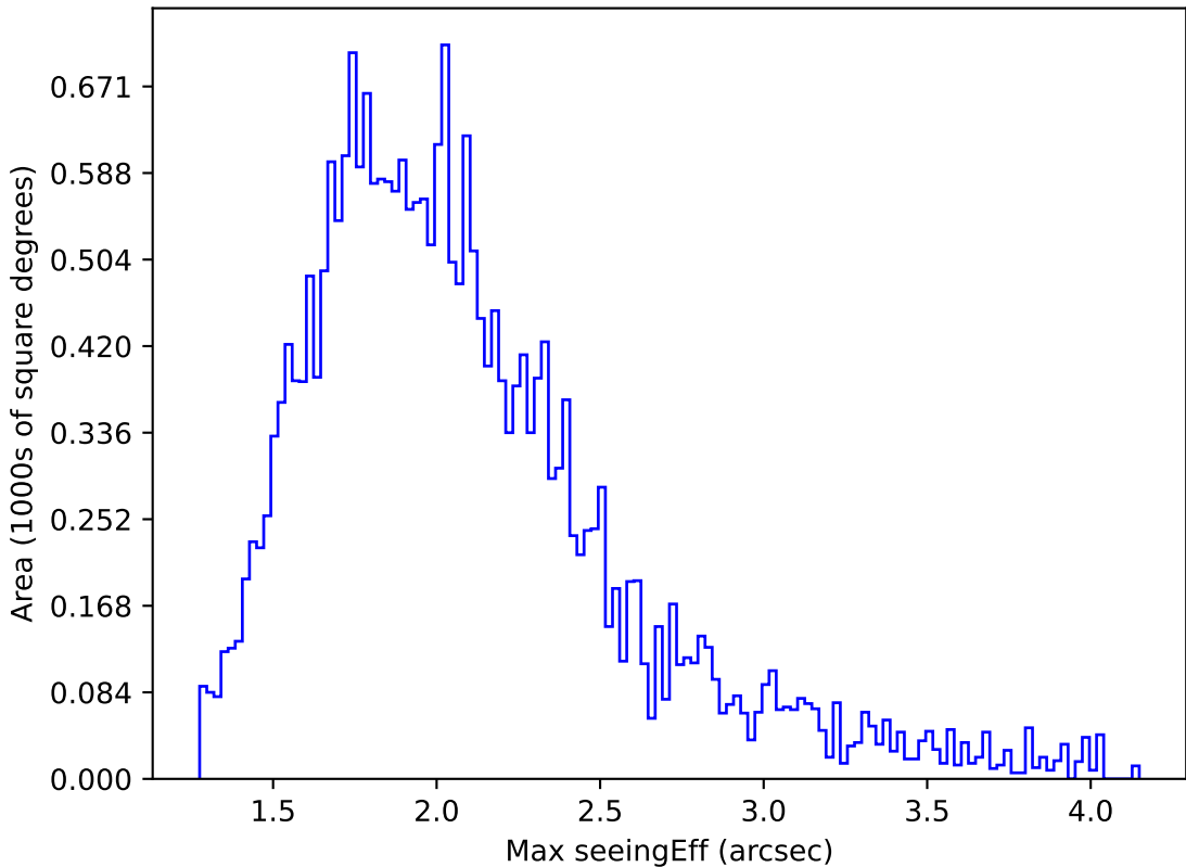
too_elab_r64_d2_gz_v3.4_10yrs Yr 1 all bands: Max seeingEff
