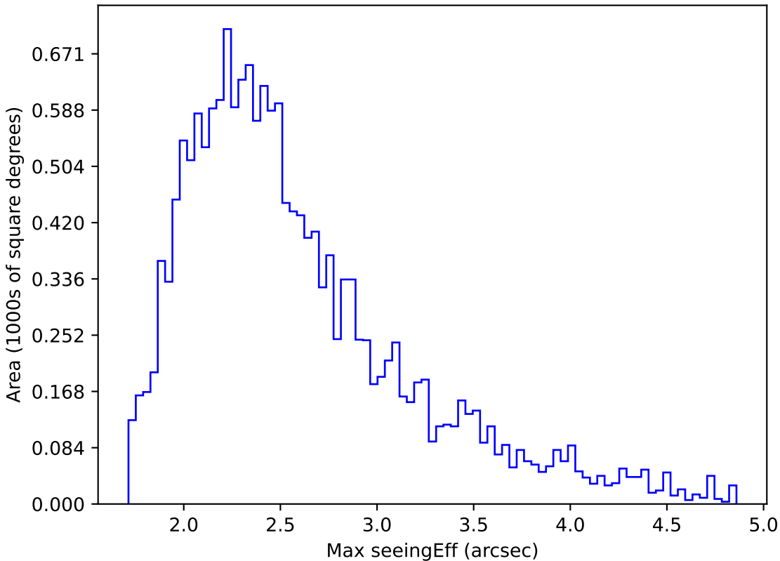
too_elab_r64_d2_gz_v3.4_10yrs WFD z band: Max seeingEff
