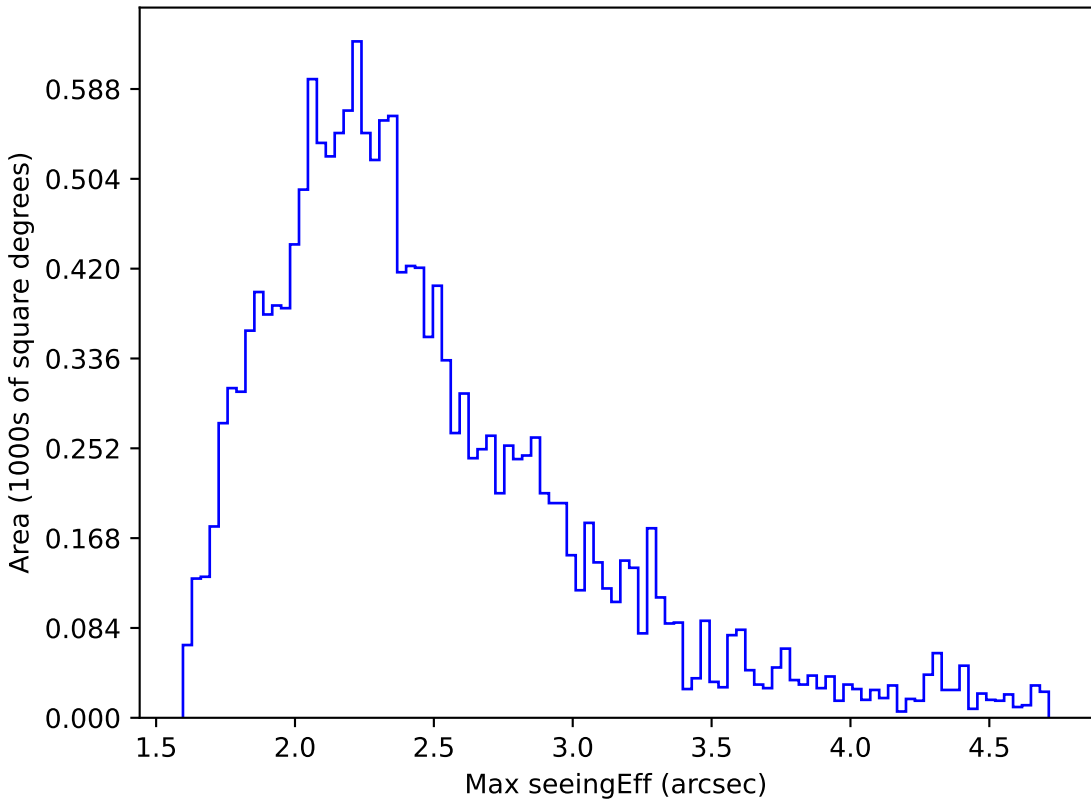
too_elab_r64_d2_gz_v3.4_10yrs WFD y band: Max seeingEff
