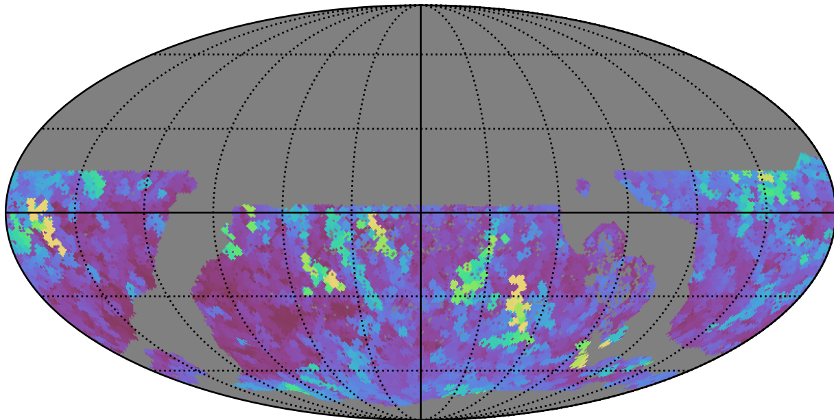
too_elab_r64_d2_gz_v3.4_10yrs WFD i band: Max seeingEff
