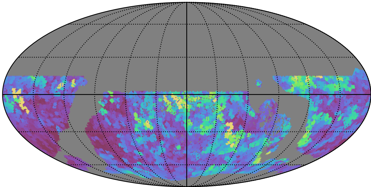
too_elab_r64_d2_gz_v3.4_10yrs WFD all bands: Max seeingEff
