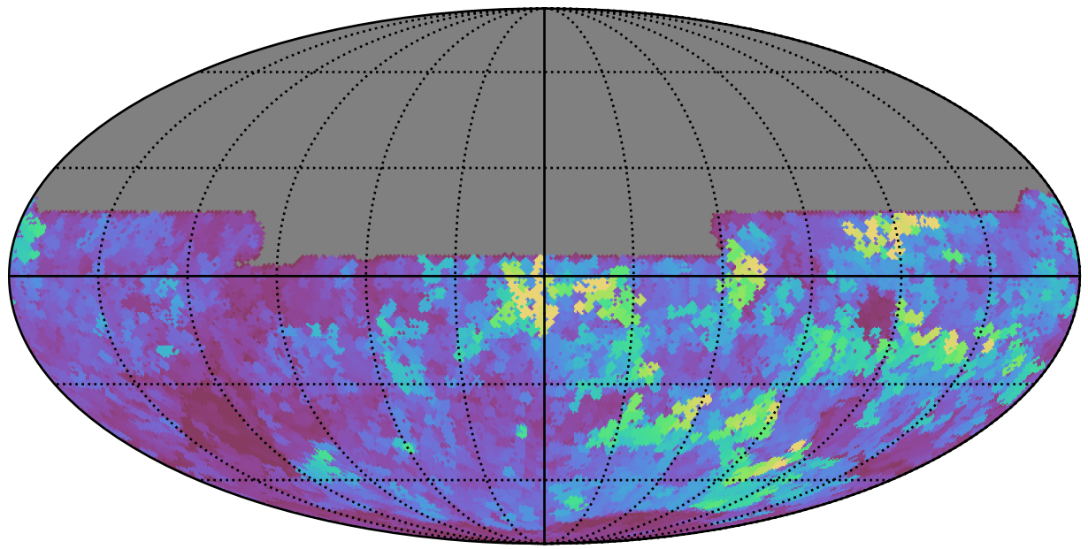
too_elab_r64_d2_gz_v3.4_10yrs All sky y band: Max seeingEff
