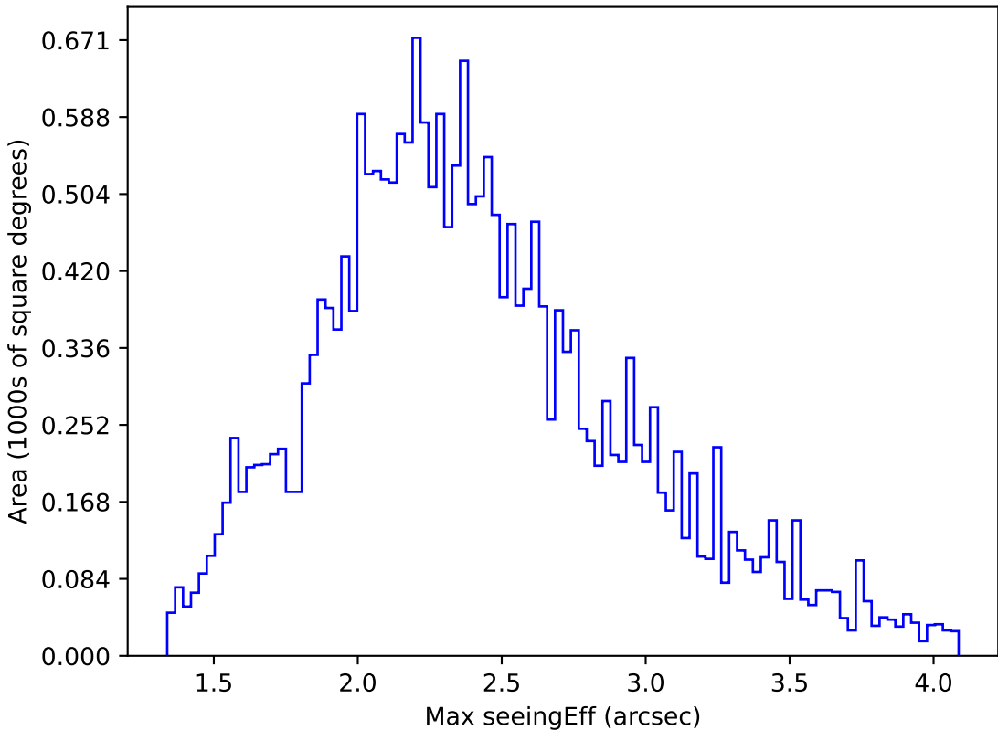
too_elab_r64_d2_gz_v3.4_10yrs All sky u band: Max seeingEff
