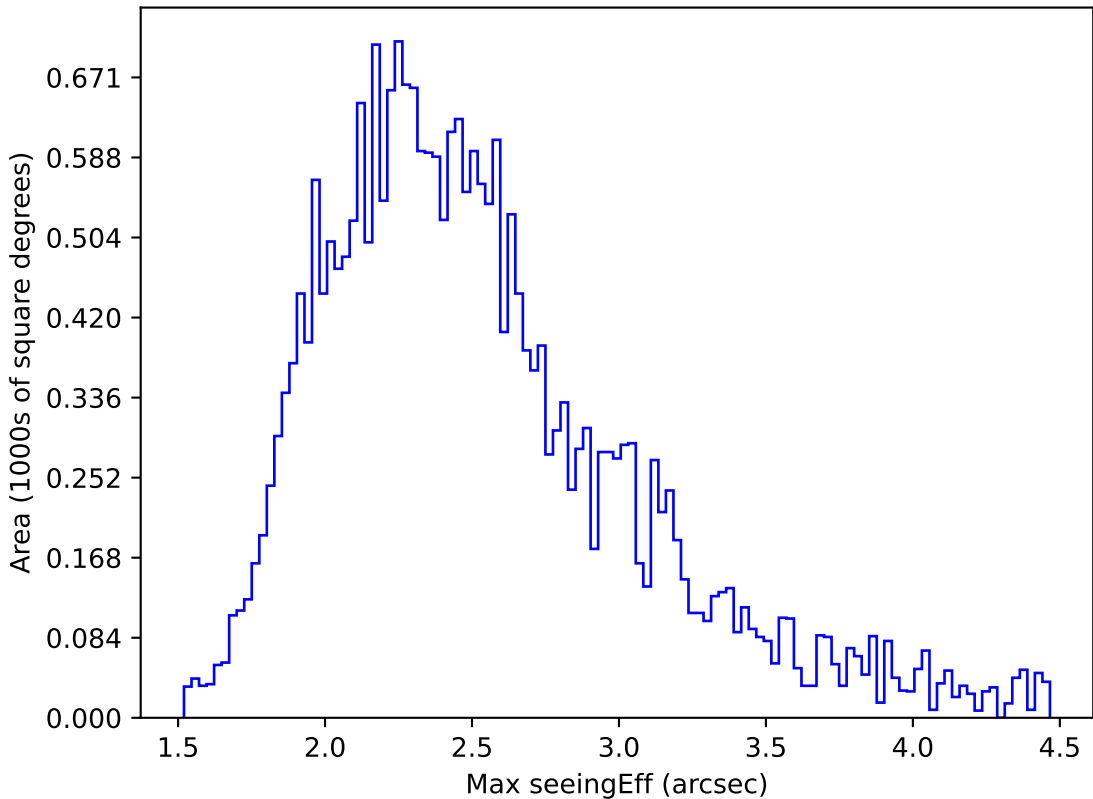
too_elab_r64_d2_gz_v3.4_10yrs All sky g band: Max seeingEff
