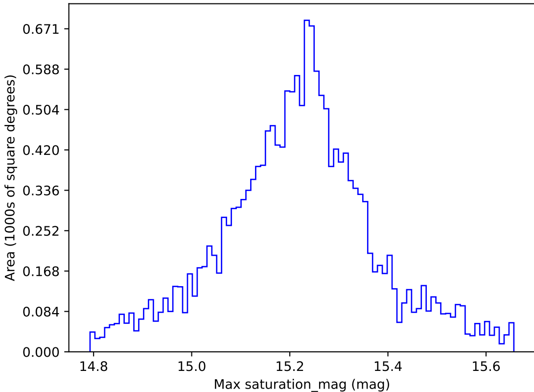
too_elab_r64_d2_gz_v3.4_10yrs WFD z band: Max saturation_mag
