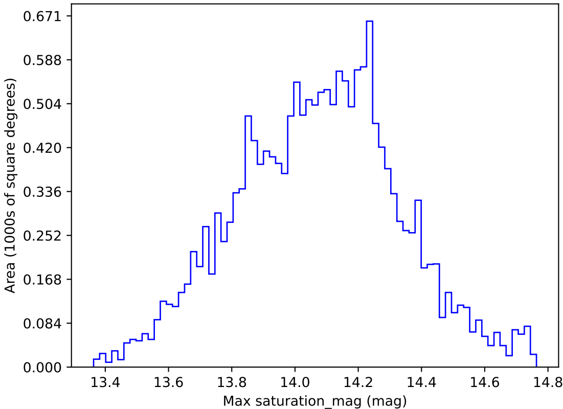
too_elab_r64_d2_gz_v3.4_10yrs WFD u band: Max saturation_mag
