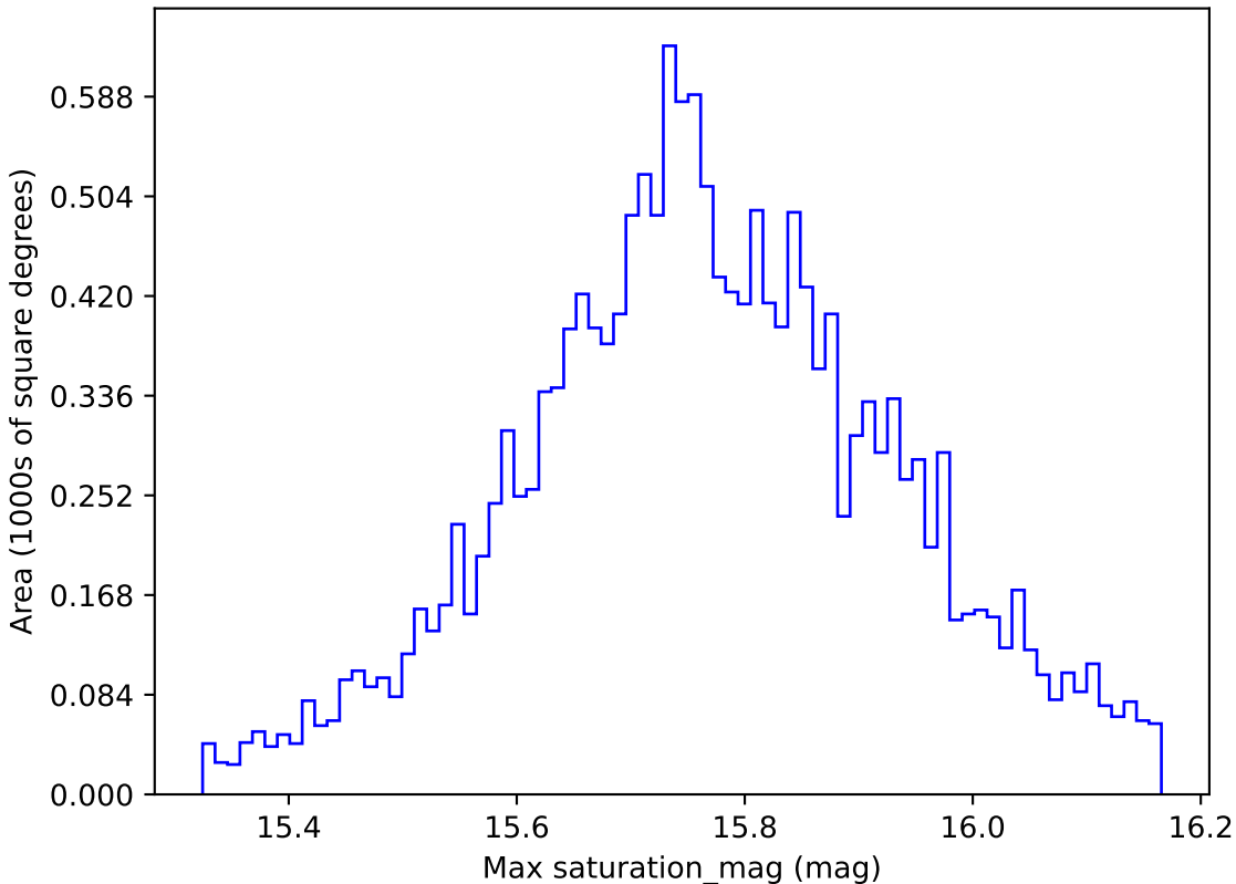
too_elab_r64_d2_gz_v3.4_10yrs WFD r band: Max saturation_mag
