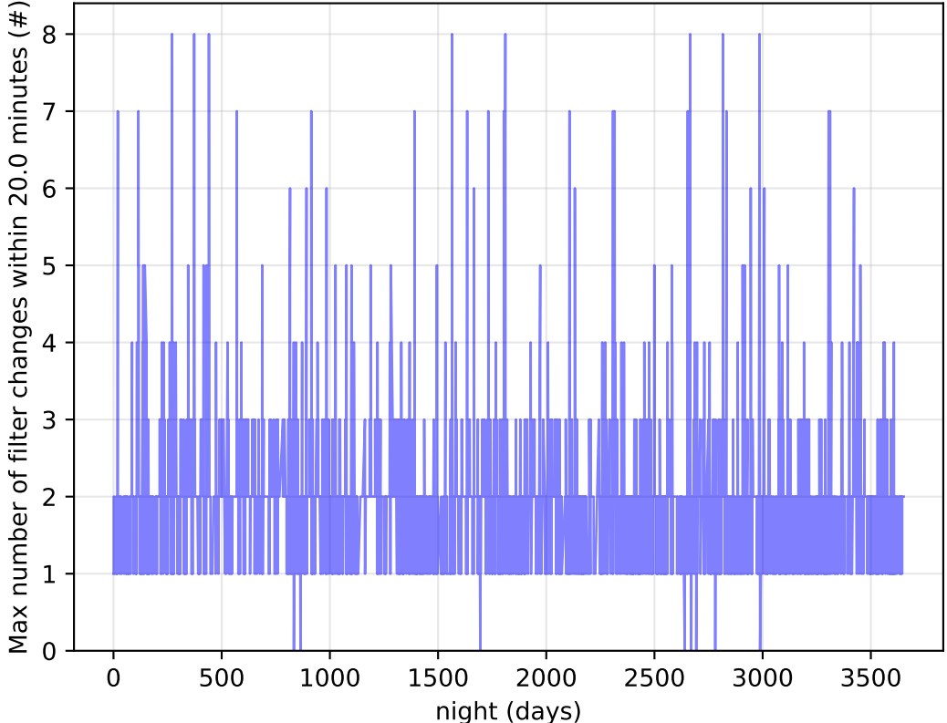
too_elab_r64_d2_gz_v3.4_10yrs Per Night: Max number of filter changes within 20.0 minutes
