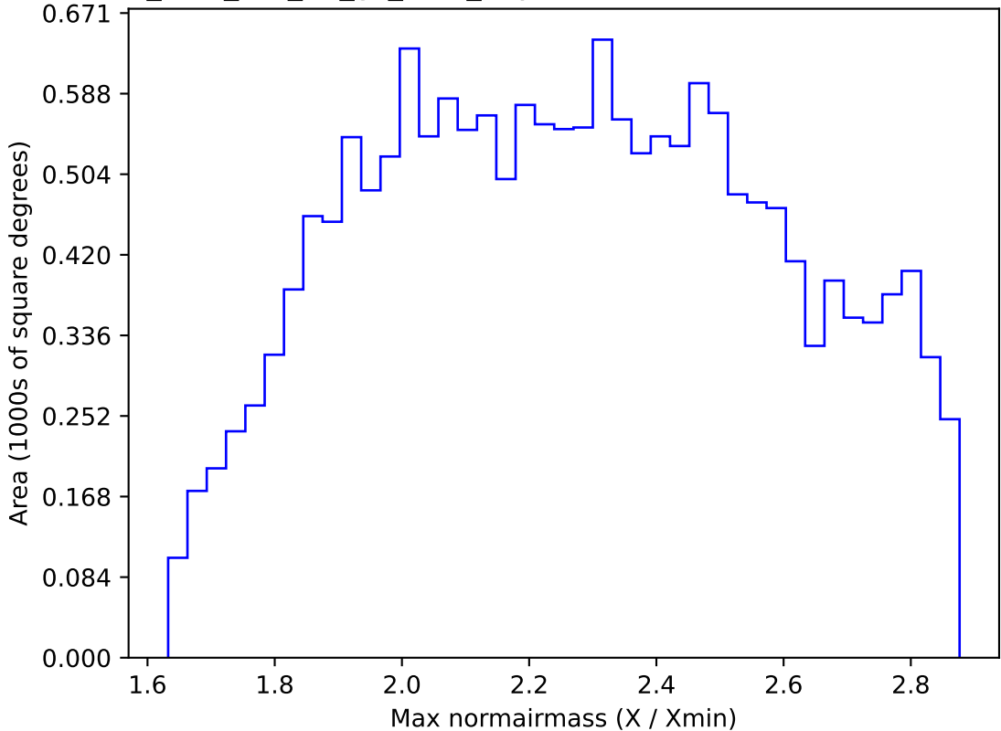
too_elab_r64_d2_gz_v3.4_10yrs WFD z band: Max normairmass
