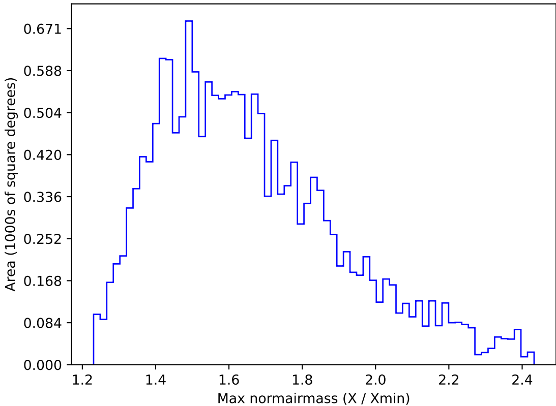
too_elab_r64_d2_gz_v3.4_10yrs WFD u band: Max normairmass
