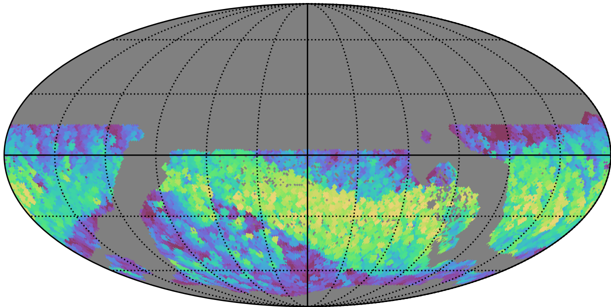
too_elab_r64_d2_gz_v3.4_10yrs WFD i band: Max normairmass
