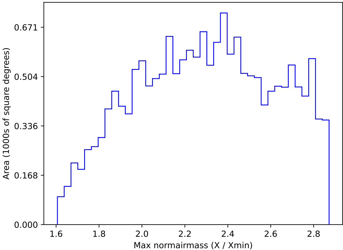
too_elab_r64_d2_gz_v3.4_10yrs WFD i band: Max normairmass
