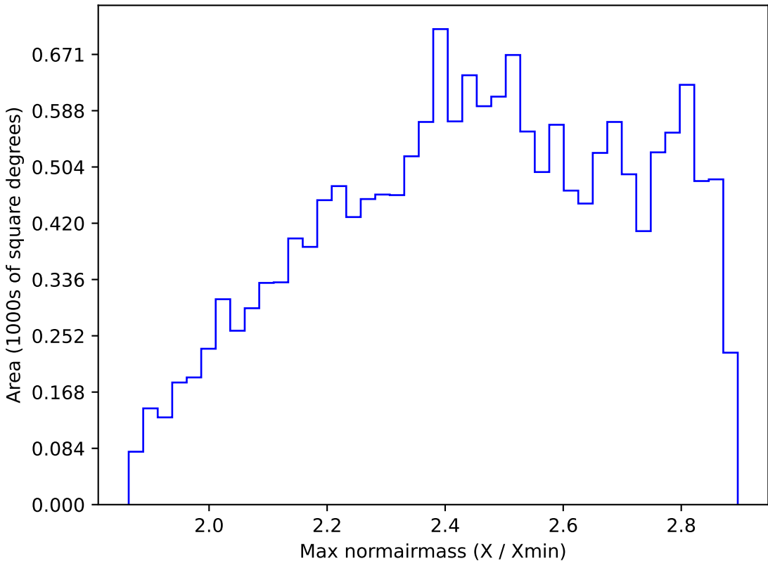
too_elab_r64_d2_gz_v3.4_10yrs WFD all bands: Max normairmass
