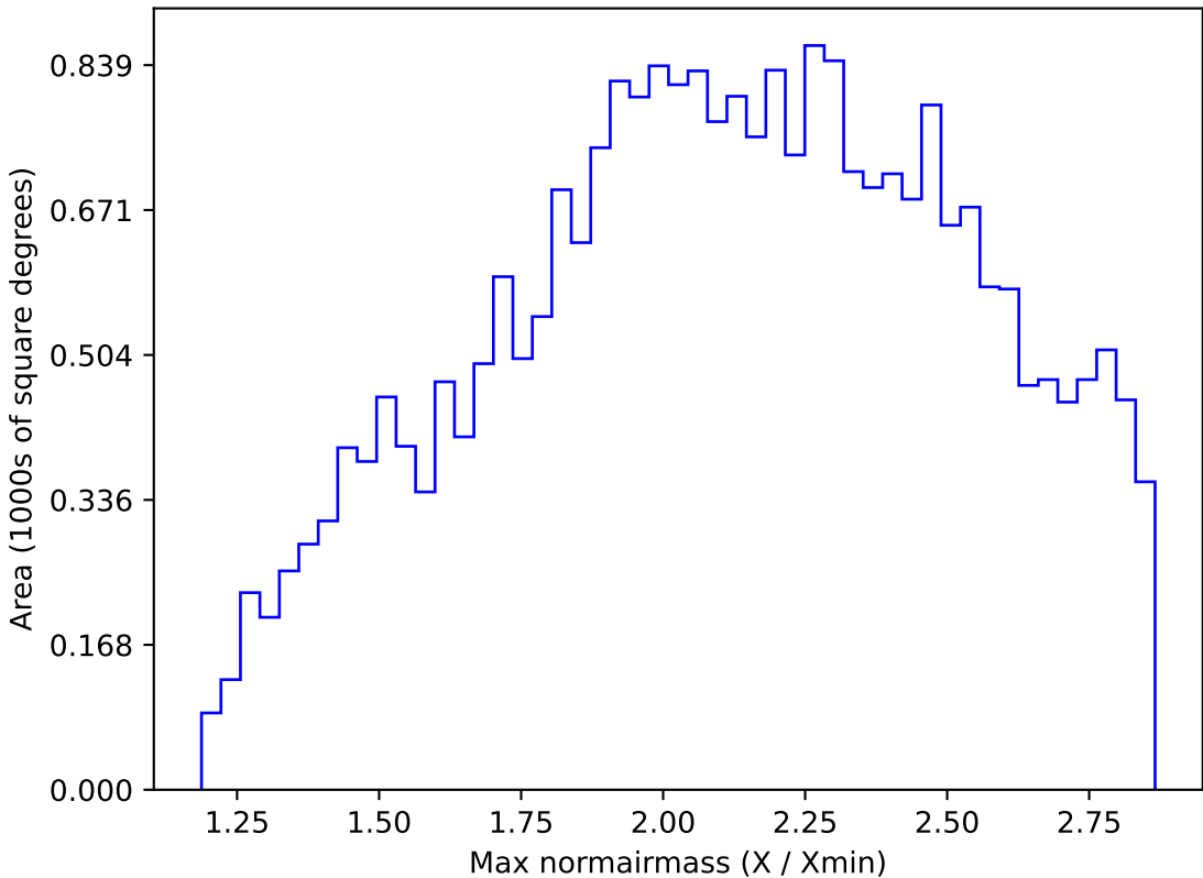
too_elab_r64_d2_gz_v3.4_10yrs All sky z band: Max normairmass
