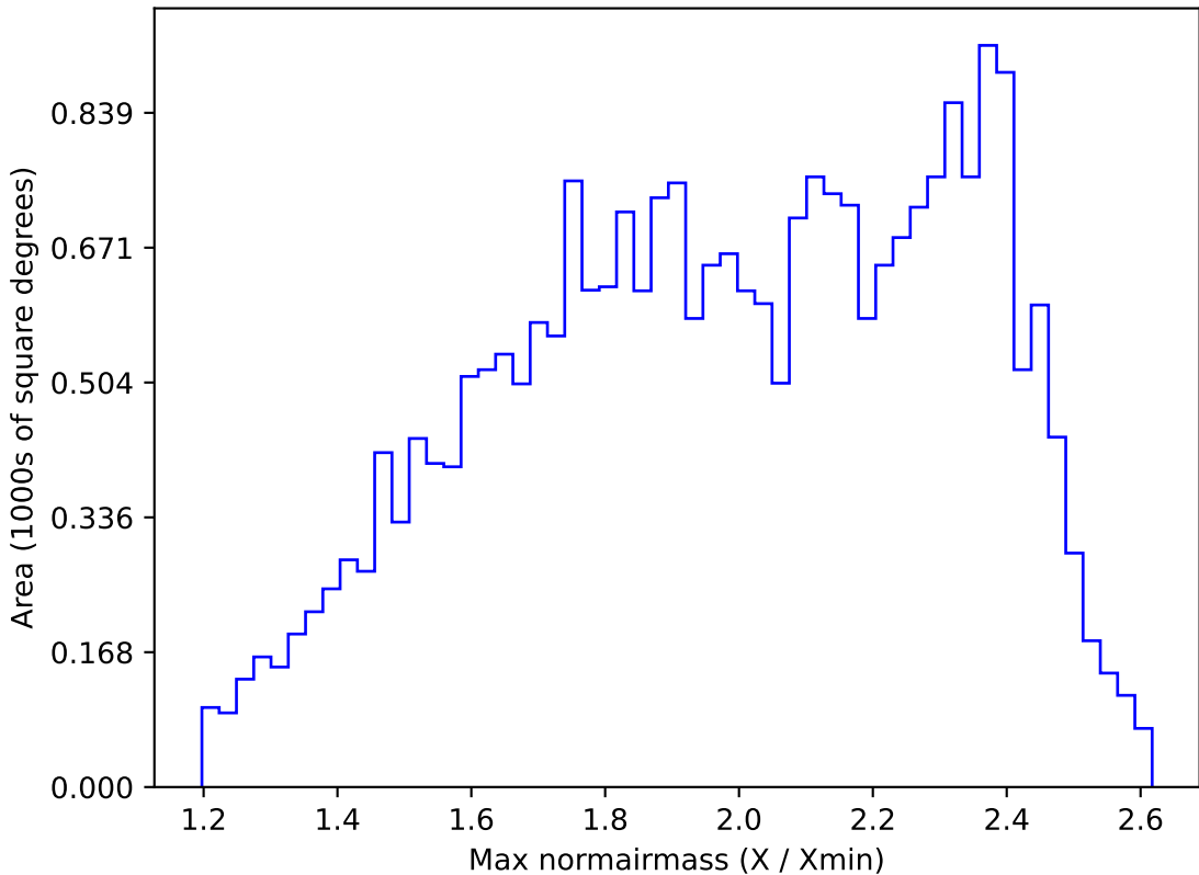
too_elab_r64_d2_gz_v3.4_10yrs All sky r band: Max normairmass
