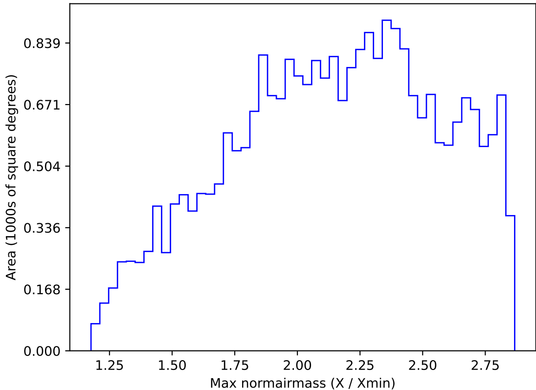
too_elab_r64_d2_gz_v3.4_10yrs All sky i band: Max normairmass
