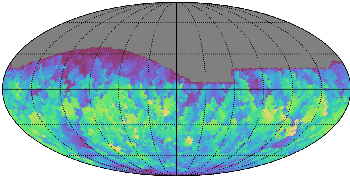
too_elab_r64_d2_gz_v3.4_10yrs All sky g band: Max normairmass
