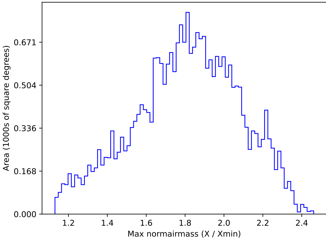
too_elab_r64_d2_gz_v3.4_10yrs All sky g band: Max normairmass
