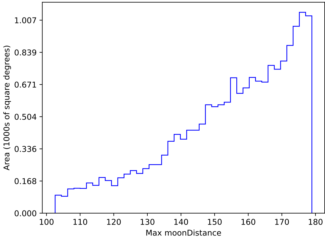
too_elab_r64_d2_gz_v3.4_10yrs WFD z band: Max moonDistance
