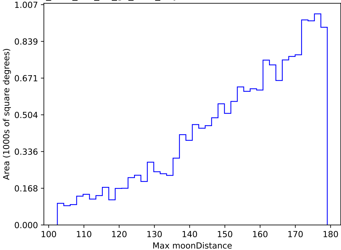
too_elab_r64_d2_gz_v3.4_10yrs WFD u band: Max moonDistance
