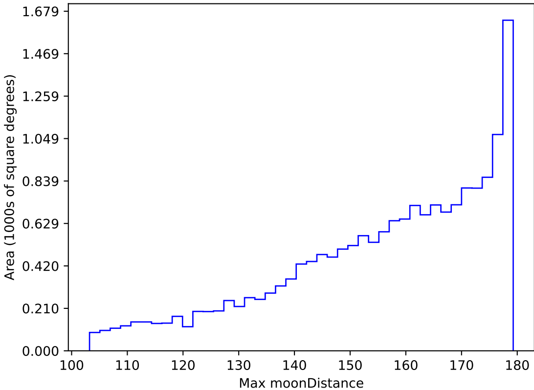
too_elab_r64_d2_gz_v3.4_10yrs WFD r band: Max moonDistance
