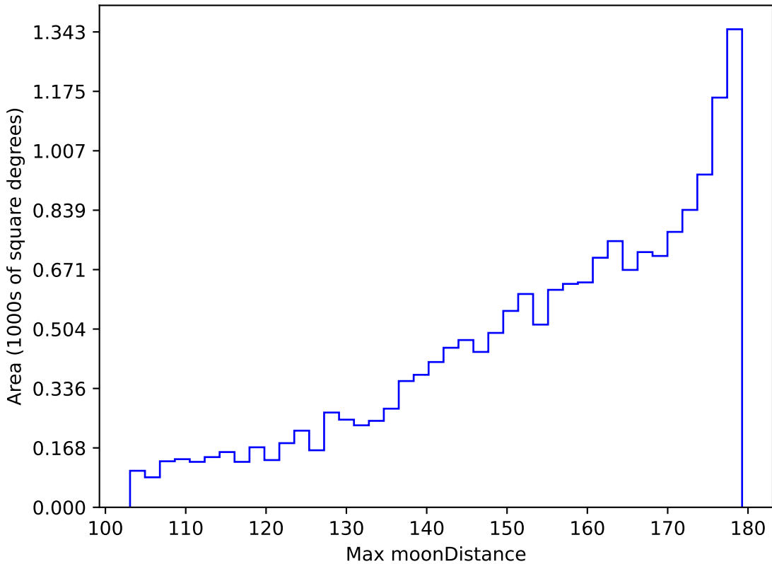
too_elab_r64_d2_gz_v3.4_10yrs WFD i band: Max moonDistance
