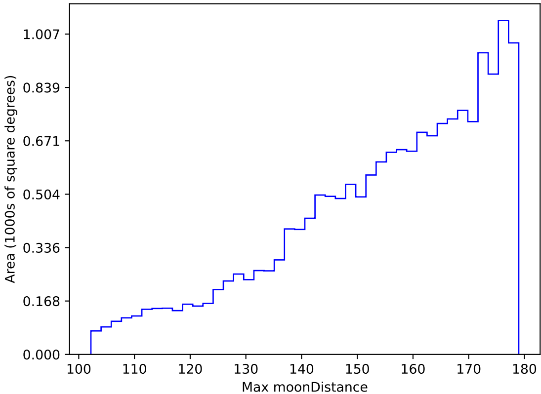
too_elab_r64_d2_gz_v3.4_10yrs WFD g band: Max moonDistance
