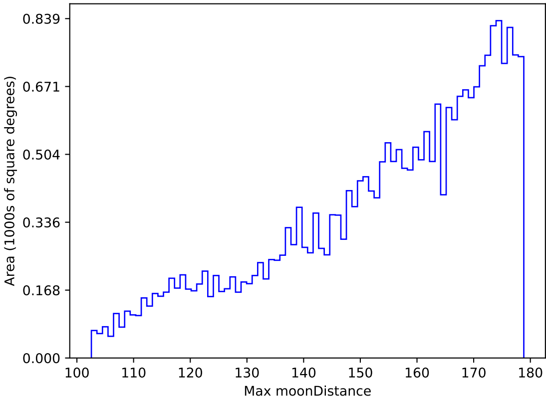
too_elab_r64_d2_gz_v3.4_10yrs All sky z band: Max moonDistance
