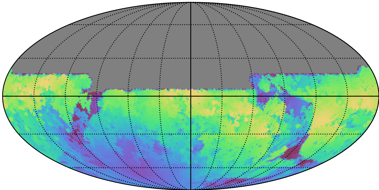
too_elab_r64_d2_gz_v3.4_10yrs All sky y band: Max moonDistance
