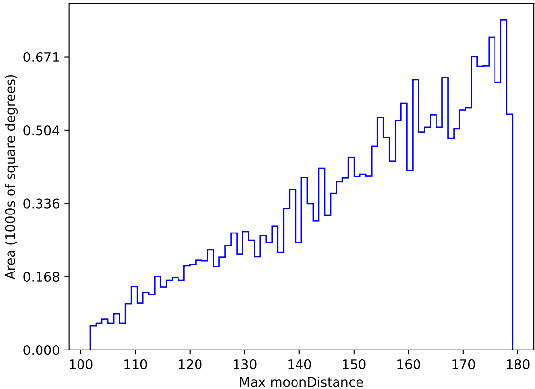
too_elab_r64_d2_gz_v3.4_10yrs All sky u band: Max moonDistance
