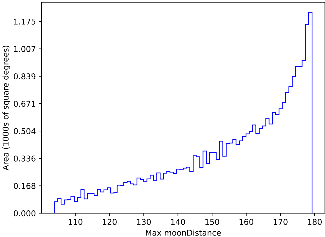
too_elab_r64_d2_gz_v3.4_10yrs All sky r band: Max moonDistance
