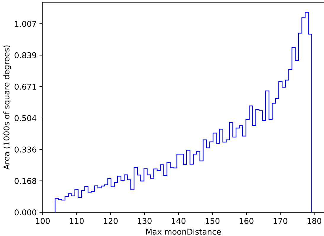
too_elab_r64_d2_gz_v3.4_10yrs All sky i band: Max moonDistance
