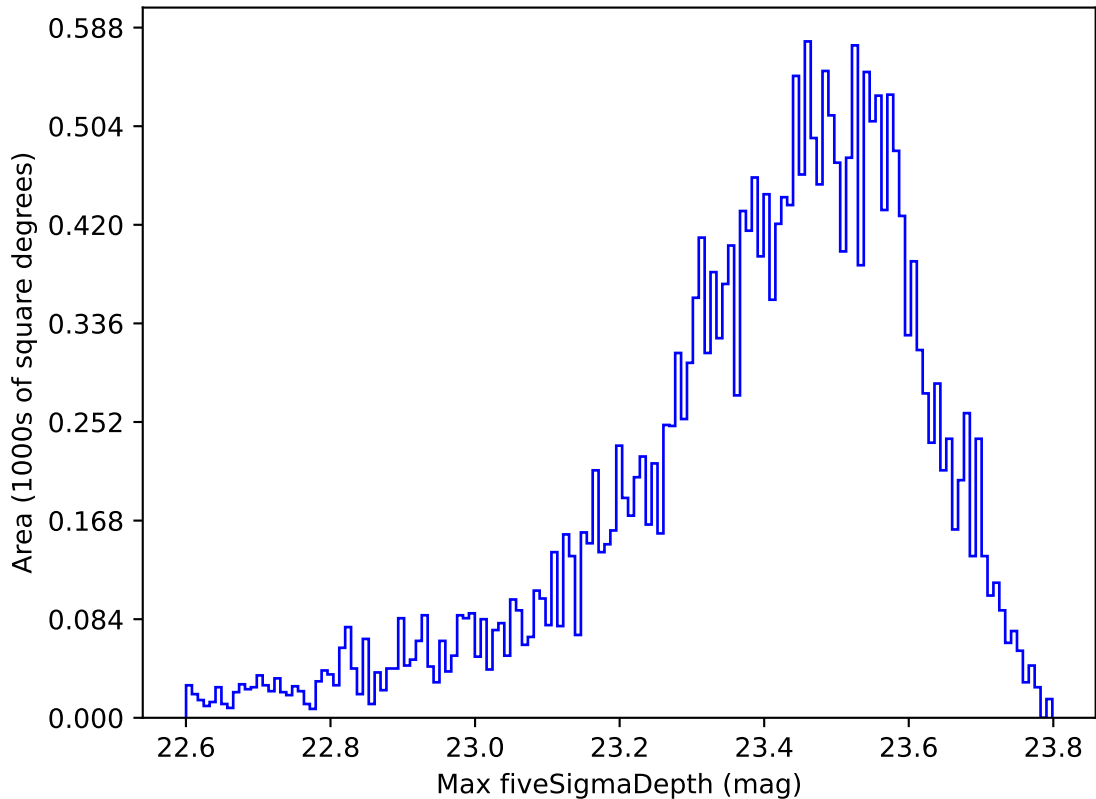
too_elab_r64_d2_gz_v3.4_10yrs Yr 1 z band: Max fiveSigmaDepth
