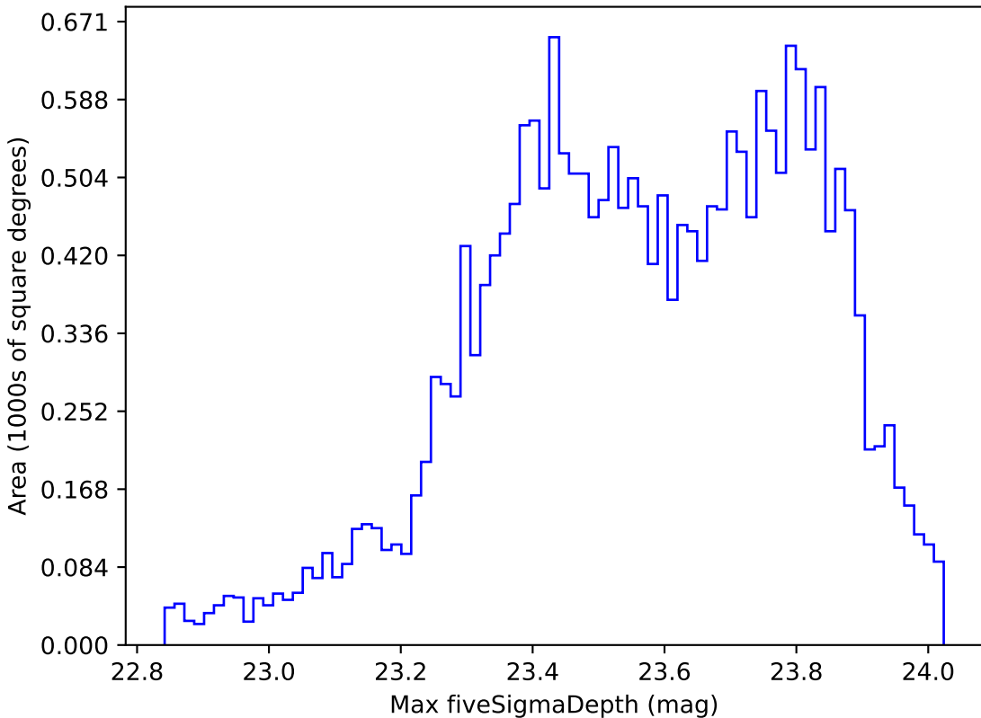
too_elab_r64_d2_gz_v3.4_10yrs Yr 1 u band: Max fiveSigmaDepth
