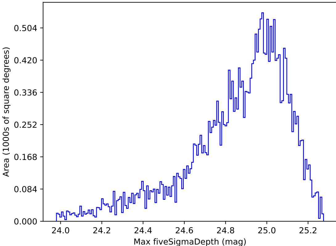
too_elab_r64_d2_gz_v3.4_10yrs Yr 1 g band: Max fiveSigmaDepth
