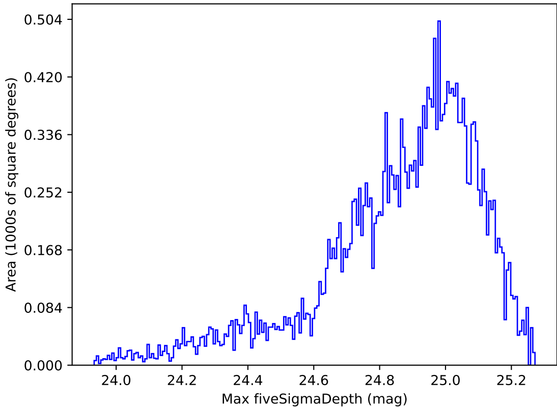
too_elab_r64_d2_gz_v3.4_10yrs Yr 1 all bands: Max fiveSigmaDepth
