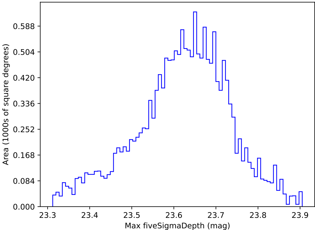
too_elab_r64_d2_gz_v3.4_10yrs WFD z band: Max fiveSigmaDepth
