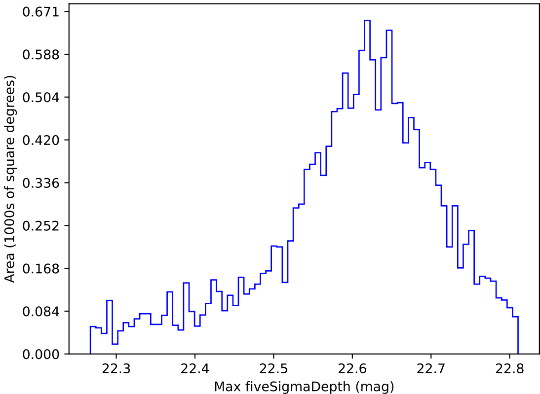
too_elab_r64_d2_gz_v3.4_10yrs WFD y band: Max fiveSigmaDepth
