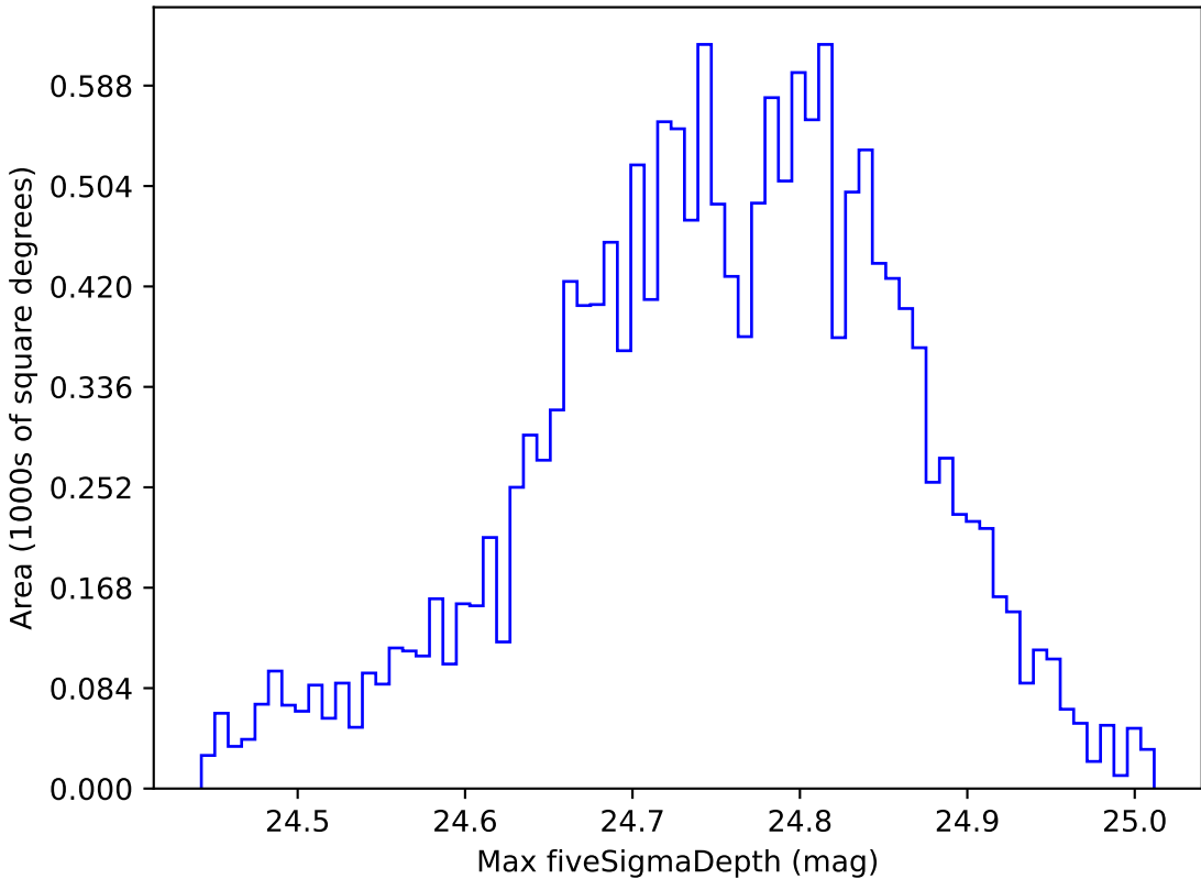
too_elab_r64_d2_gz_v3.4_10yrs WFD r band: Max fiveSigmaDepth
