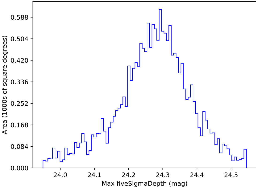
too_elab_r64_d2_gz_v3.4_10yrs WFD i band: Max fiveSigmaDepth
