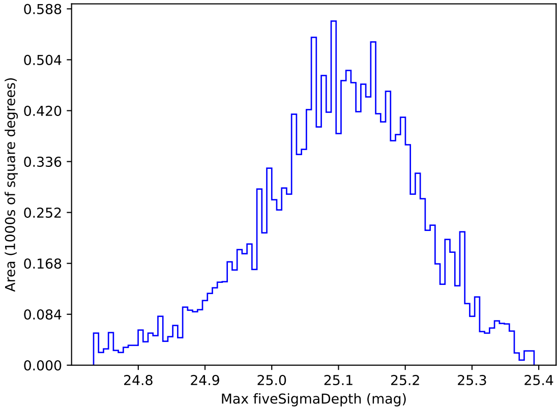
too_elab_r64_d2_gz_v3.4_10yrs WFD g band: Max fiveSigmaDepth
