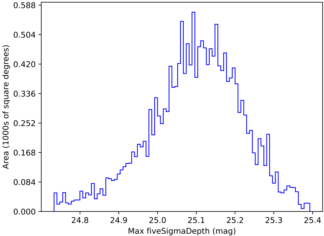
too_elab_r64_d2_gz_v3.4_10yrs WFD all bands: Max fiveSigmaDepth
