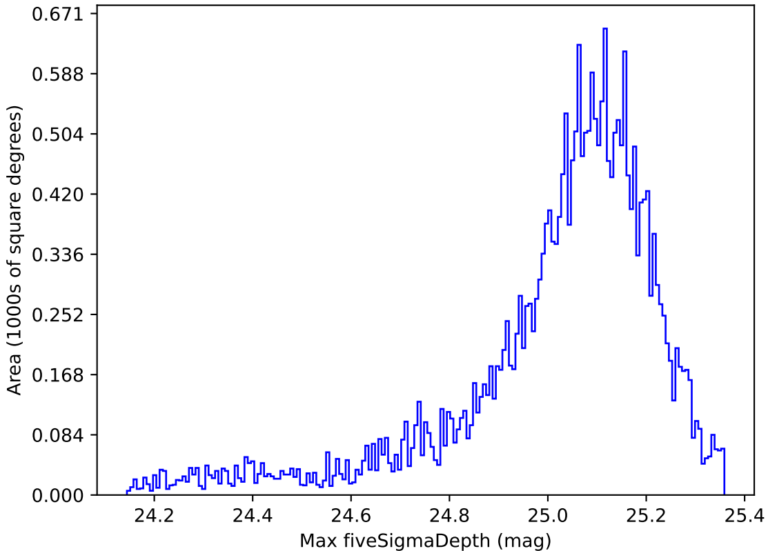
too_elab_r64_d2_gz_v3.4_10yrs All sky g band: Max fiveSigmaDepth
