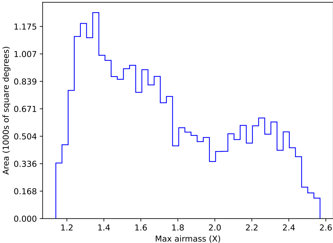
too_elab_r64_d2_gz_v3.4_10yrs Yr 1 r band: Max airmass
