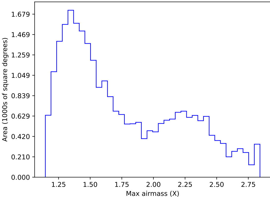
too_elab_r64_d2_gz_v3.4_10yrs Yr 1 i band: Max airmass
