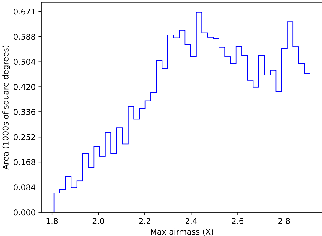
too_elab_r64_d2_gz_v3.4_10yrs WFD z band: Max airmass
